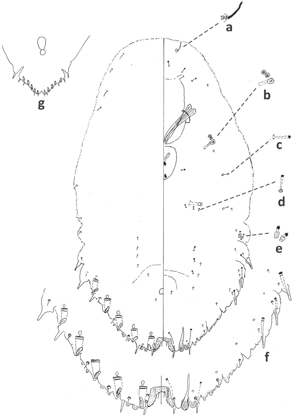
Figure 12. Fiorinia phantasma , second-instar female and second-instar female shed skin, Palm Beach Co., Boynton Beach, November 6, 2019, on Wodyetia bifurcata , (2019-6182). Abbreviations: a) antenna; b) anterior spiracle; c) microduct with sclerotized orifice; g) old second-instar female, Philippines, June 28, 1996 on Plumeria sp., 2 nd ♀ (SF023635).
