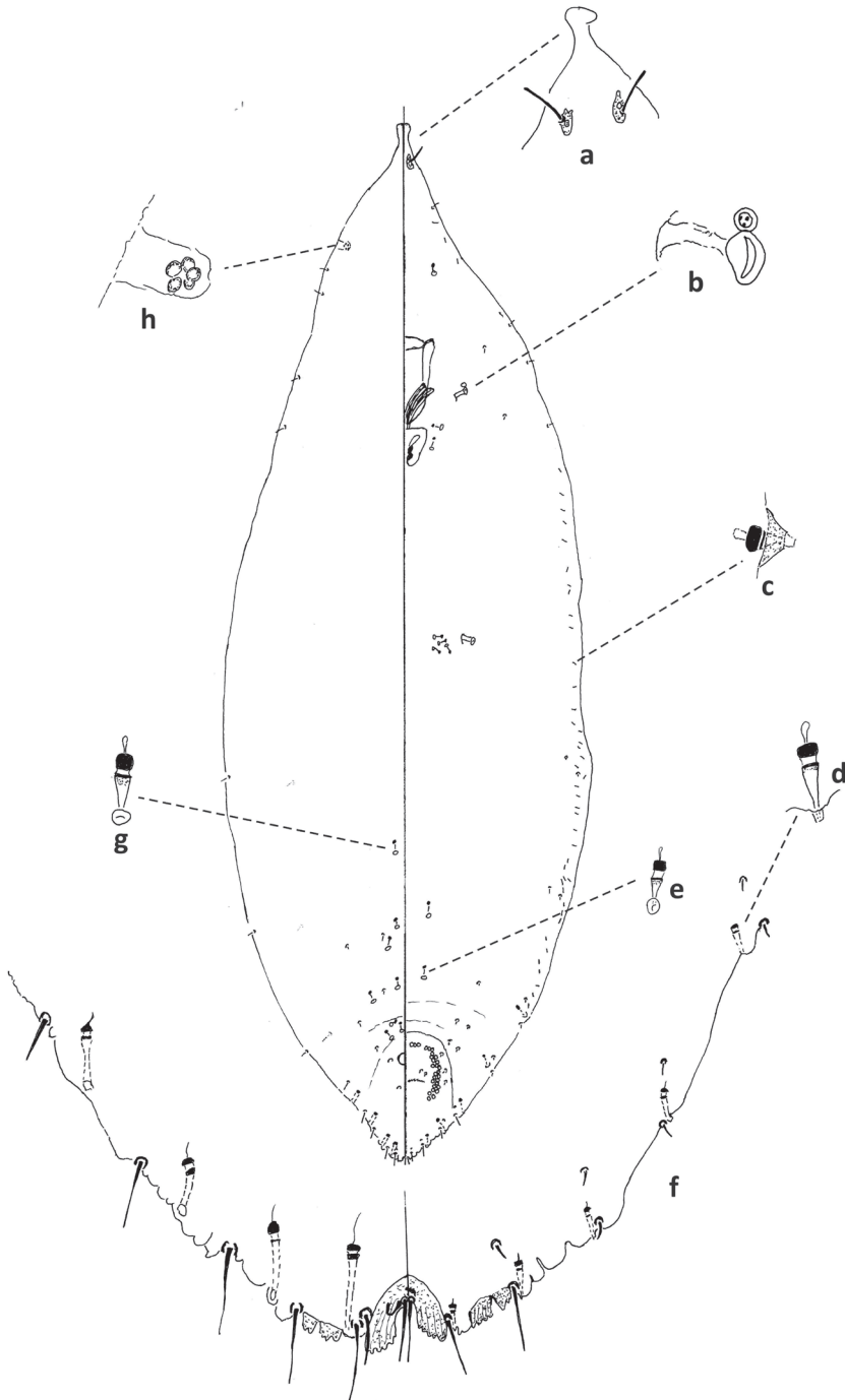
Figure 17. Fiorinia proboscidea , adult female, Hillsborough Co., Tampa, December 16, 2013, on Citrus sp., J. Hoffman (2013-9087). Abbreviations: a) conical head with protrusion, antennae; b) anterior spiracle; c) gland tubercle; d) gland spine with small dermal protrusion; e) small microduct; f) enlargement of pygidium; g) microduct; h) circular tubercles in invagination.
