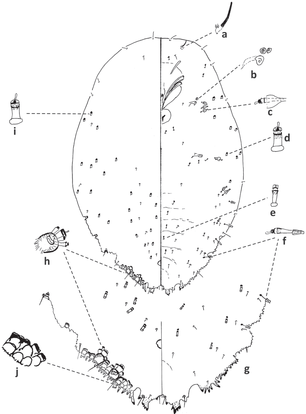
Figure 9. Fiorinia japonica , second-instar male Virginia, Chesterfield Co., Southside Nursey, July 27, 1974, on blue spruce, R. Sears. Abbreviations: a) antenna; b) anterior spiracle; c) large gland spine; d) large microduct; e) small microduct; f) small gland spine; g) enlargement of pygidium; h) enlargement of portion of duct cluster; i) large microduct; j) enlargement of communal duct.
