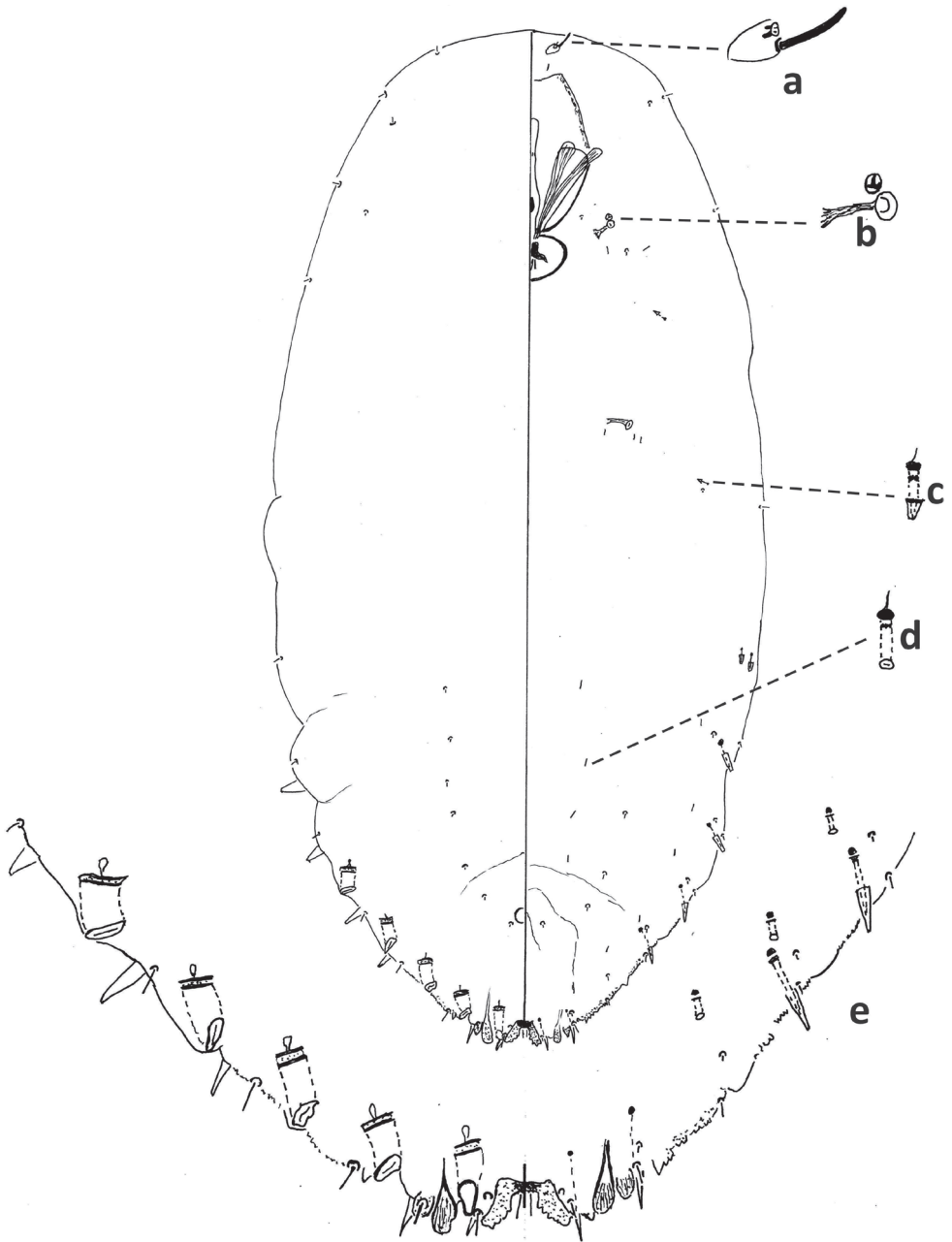
Figure 8. Fiorinia japonica second-instar female, Virginia, Chesterfield Co., Southside Nursey, July 27, 1974, on blue spruce, R. Sears. Abbreviations: a) antenna; b) anterior spiracle; c) microduct with sclerotized orifice; d) small microduct; e) enlargement of pygidium.
