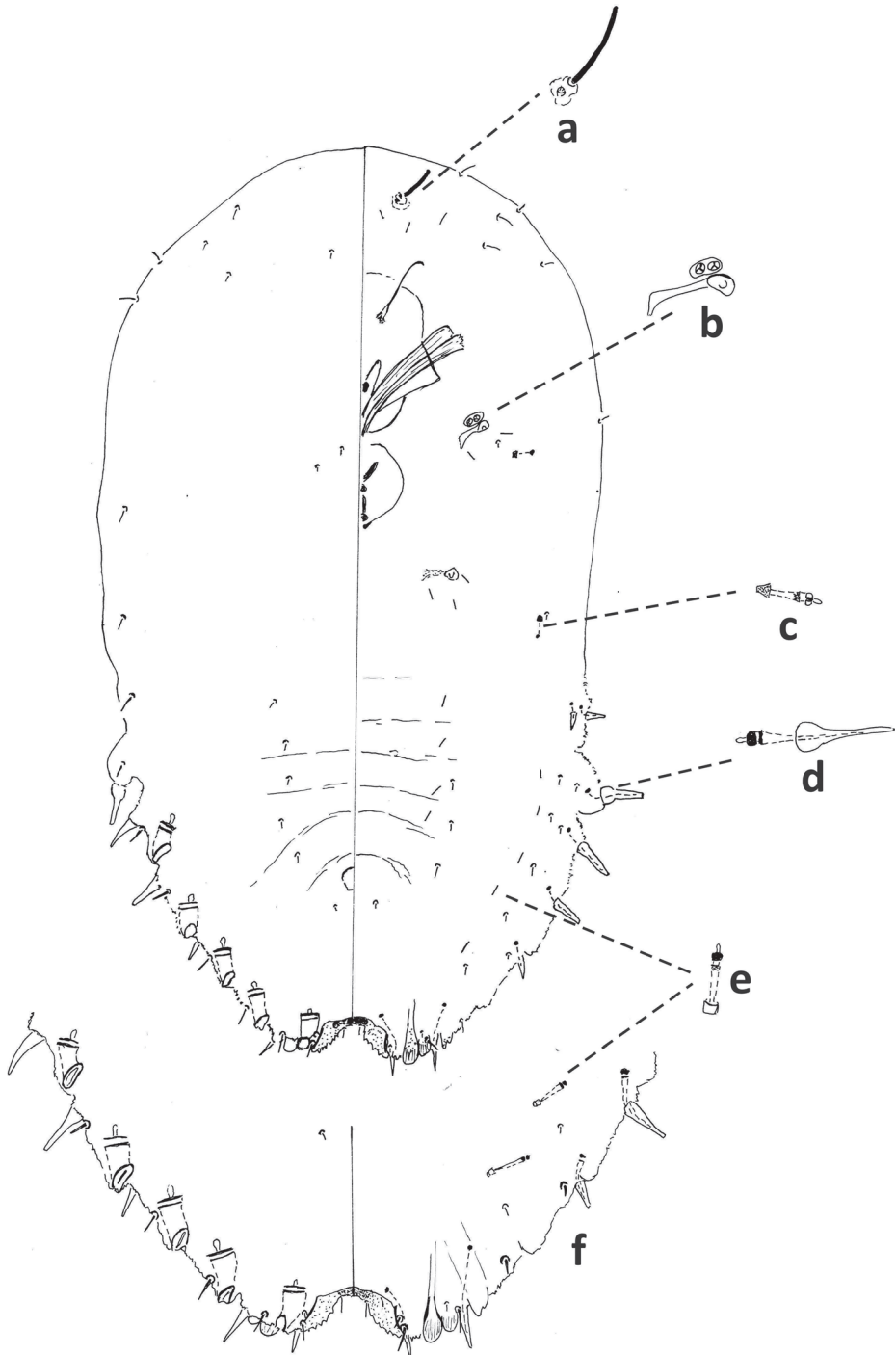
Figure 6. Fiorinia fiorinia , second-instar female, Marion Co., Ocala, August 13, 2019 on Chamaerops humilis , T. Gordon, (2019-4546). Abbreviations: a) antenna; b) anterior spiracle; c) microduct with sclerotized orifice; d) large gland spine; e) large microduct; f) enlargement of pygidium.
