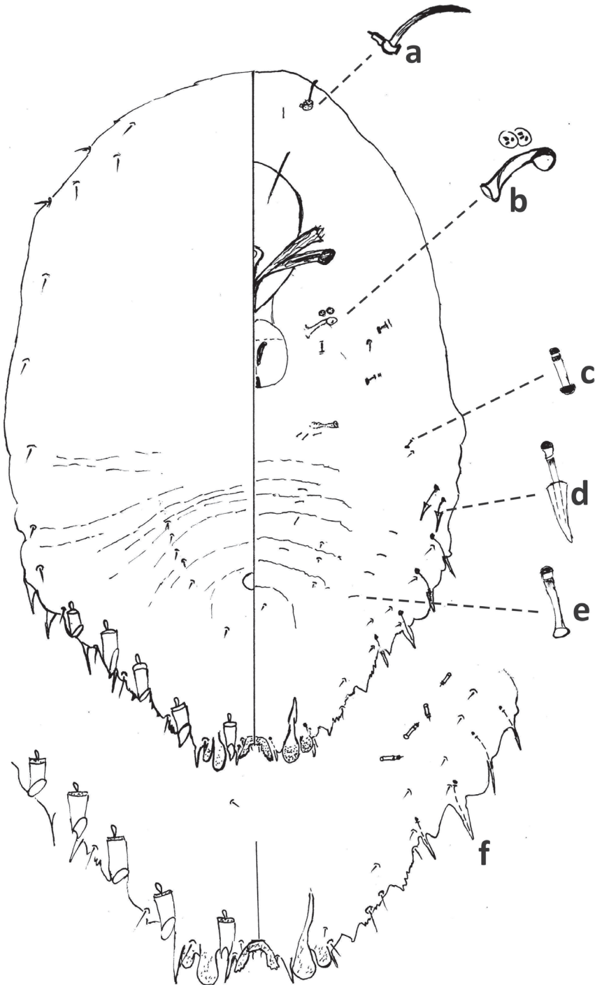
Figure 4. Fiorinia externa , second-instar female, Alleghany Co., Glade Creek, North Carolina, November 22, 2019, on Abies fraseri , A. Bartlett, (2019-6449). Abbreviations: a) antenna; b) anterior spiracle; c) microduct with sclerotized orifice; d) large gland spine; e) small microduct; f) enlargement of pygidium.
