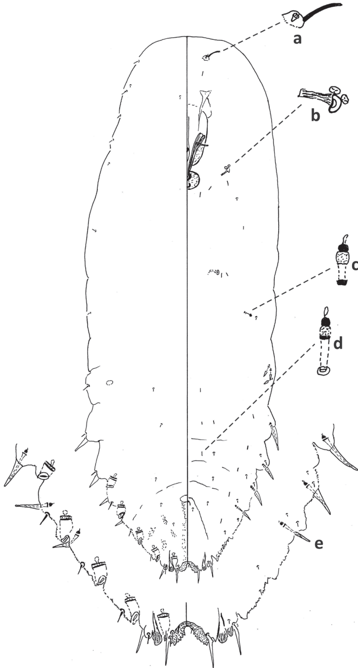
Figure 14. Fiorinia pinicola , second-instar female, Hong Kong, December 1895, on Pinus sinensis , A. Koebele (1529) mounted from type material. Abbreviations: a) antenna; b) anterior spiracle; c) small microduct with sclerotized orifice d) small microduct e) enlargement of pygidium. Note the blank blotches on the body margin of the pygidium enlargement.
