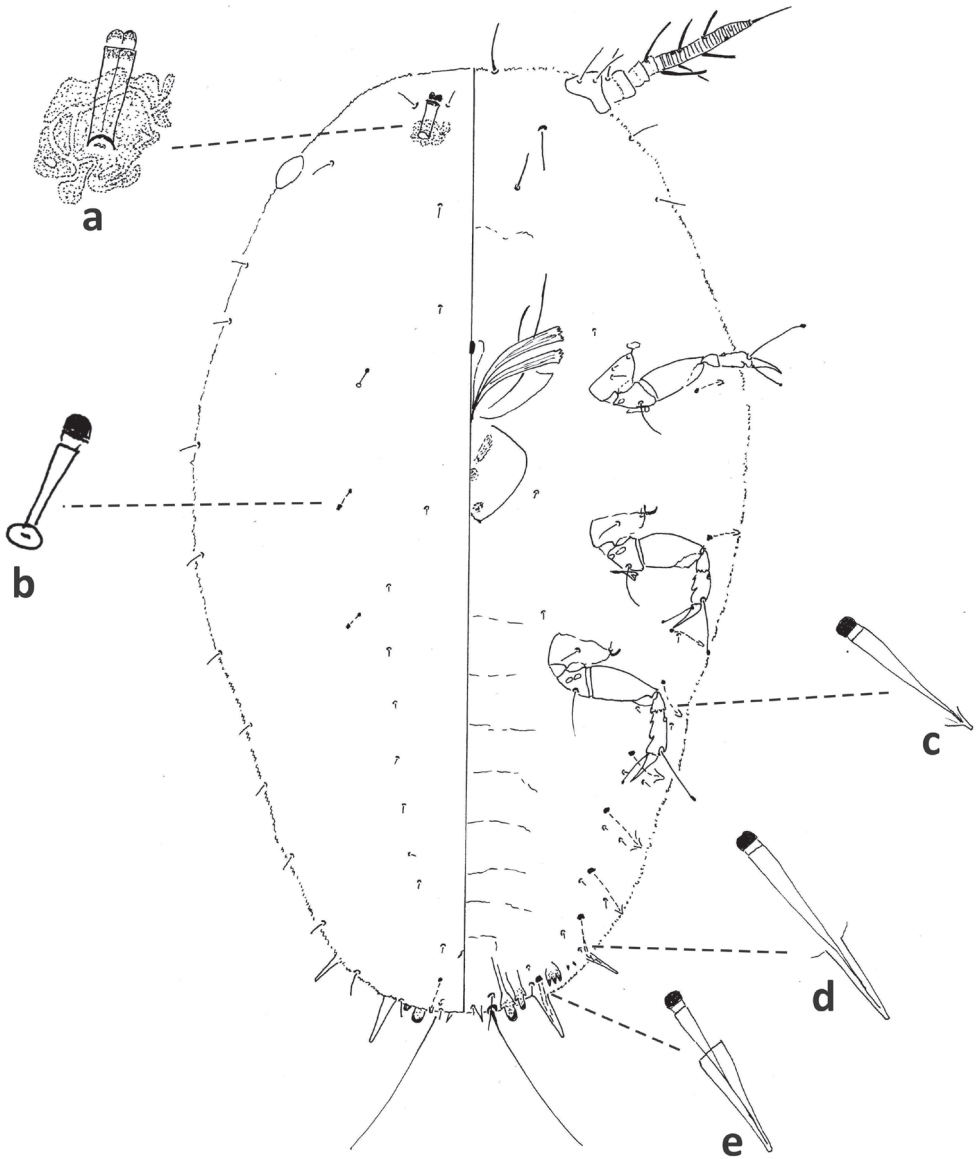
Figure 10. Fiorinia phantasma , First-instar nymph, Palm Beach Co., Boynton Beach, October 30, 2019, on Wodyetia bifurcata , L. Smith, (2019-5998). Abbreviations: a) large dorsal duct on head; b) small microduct; c) gland spine abdominal segment II with small projection; d) gland spine at abdominal segment VI with long projection; e) gland spine at abdominal segment VII with long projection.
