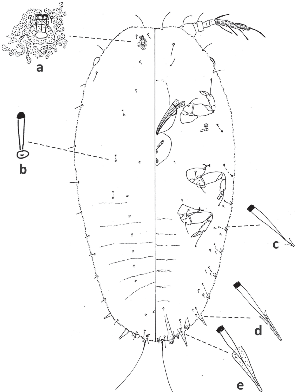
Figure 16. Fiorinia proboscidea , First-instar nymph, Putnam Co., Crescent City, October 2, 2019, on Citrus sp., D. Rigby, M. Cain, (2018-5548). Abbreviations: a) large duct on head; b) dorsal microduct; c) short gland spine on abdominal segment II; d) long gland spine on abdominal segment VI; e) long gland spine on abdominal segment VII.
