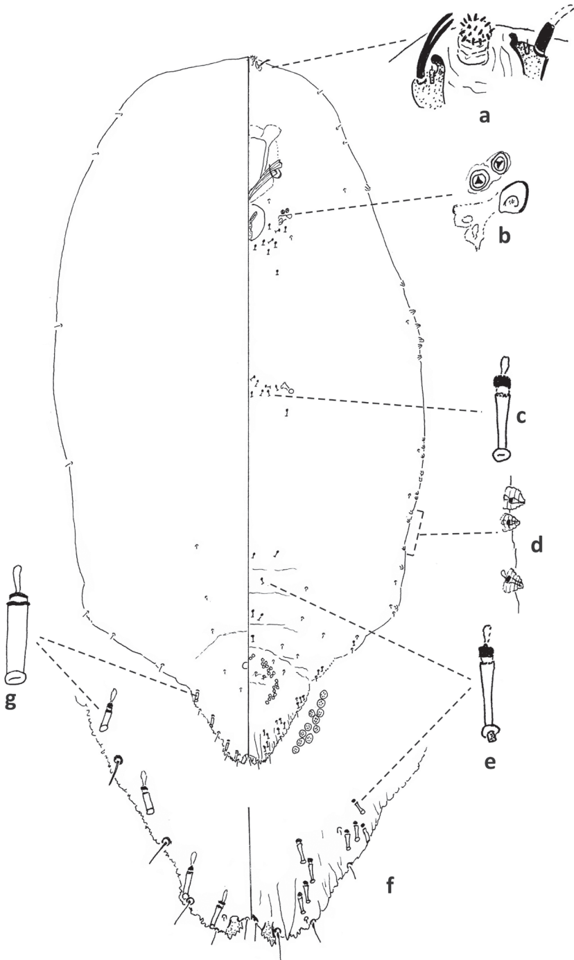
Figure 11. Fiorinia phantasma (Cockerell & Robinson); adult female, Palm Beach Co., Boynton Beach, April 6, 2020, on Ligustrum japonicum , L. Smith (2020-1365). Abbreviations: a) detail of antennae and inter-antennal process; b) detail of anterior spiracle; c) microducts; d) marginal duct tubercles; e) marginal microduct; f) detail of pygidium; g) marginal macroduct on pygidium.
