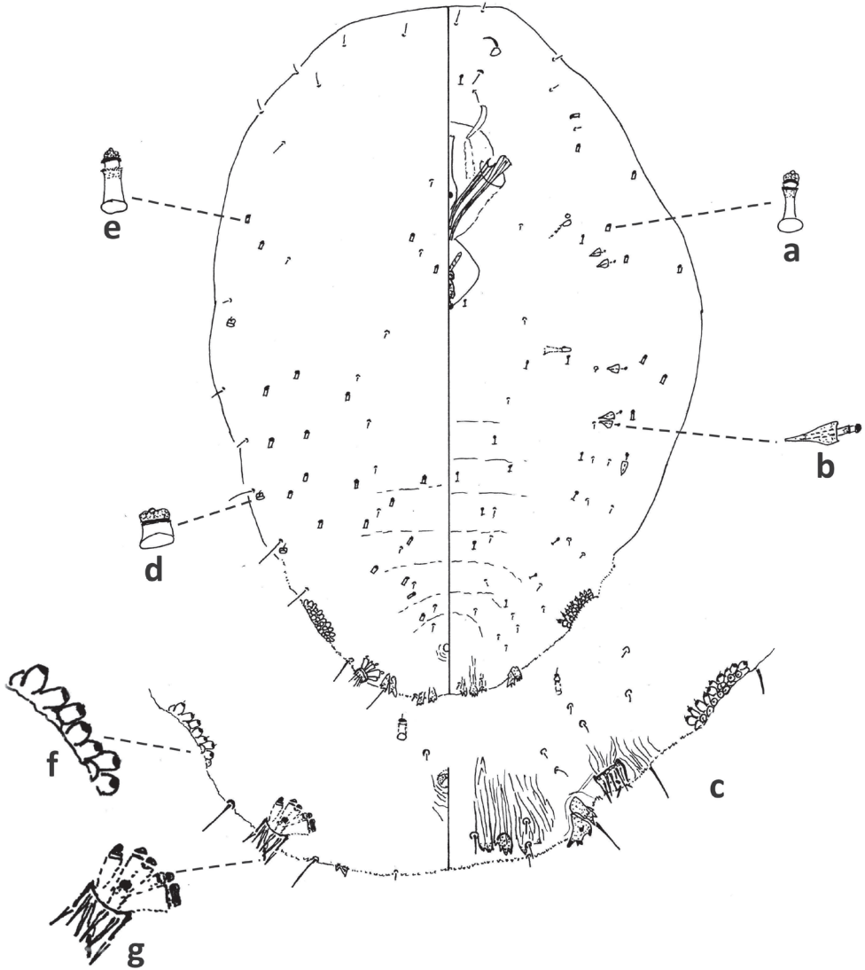
Figure 19. Fiorinia proboscidea , second-instar male, Putnam Co., Crescent City, October 2, 2019, on Citrus sp., D. Rigby, M. Cain, (2018-5548). Abbreviations: a) small microduct; b) large gland spine; c) enlargement of pygidium; d) small macroduct; e) large microduct; f) enlargement of part of duct cluster; g) enlargement of communal duct.
